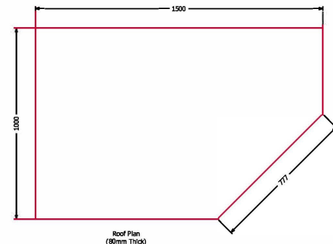
Roof Plan (90mm Thick)
