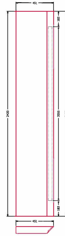
Wall Detail (90mm Thick)
