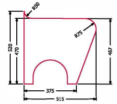
Seat Detail
