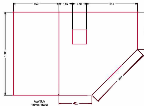
Roof Sub (90mm Thick)
