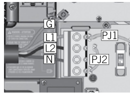
2-phase
